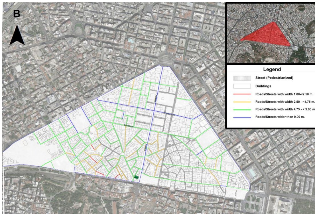
Figure 2: Roads classification (according to their width) in the Study Area.
